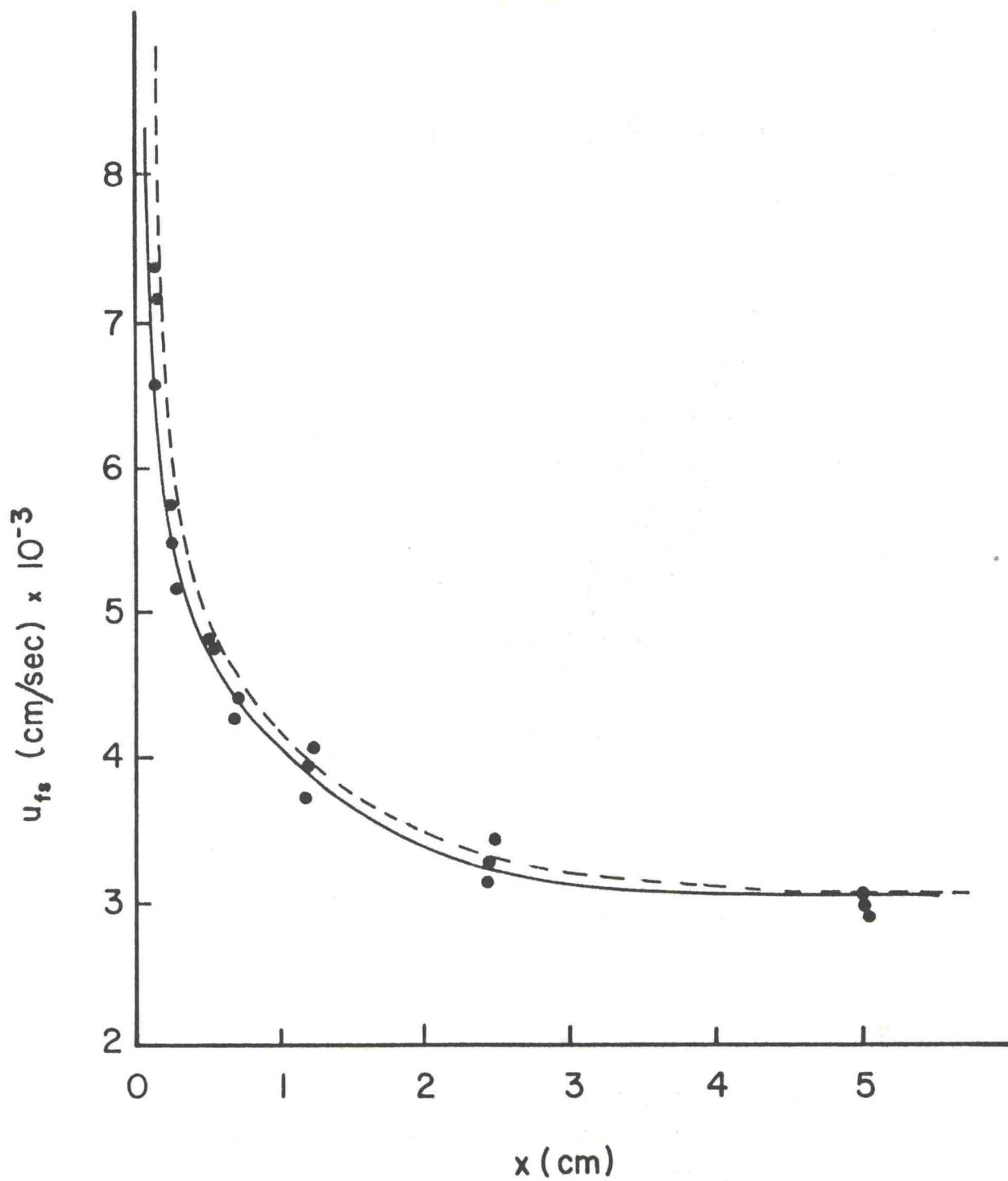
Figure 16. Decay of Precursor Amplitude in Armco Iron. Curves are fitted using Gilman dislocation velocity model. (After Taylor 40 )
